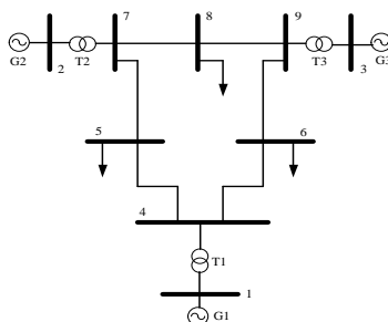
Fig. 1. WSCC 9-bus test system.
